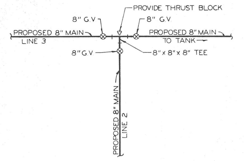
CONNECTION NO. 6 NO SCALE
