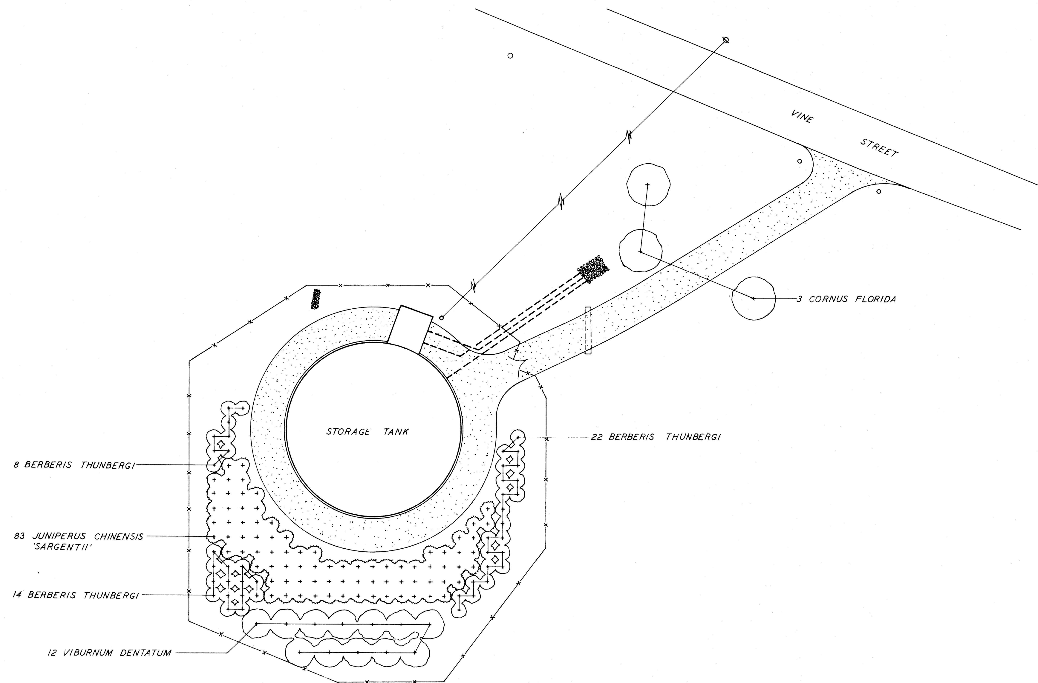
LANDSCAPING PLAN SCALE: 1"=20'
