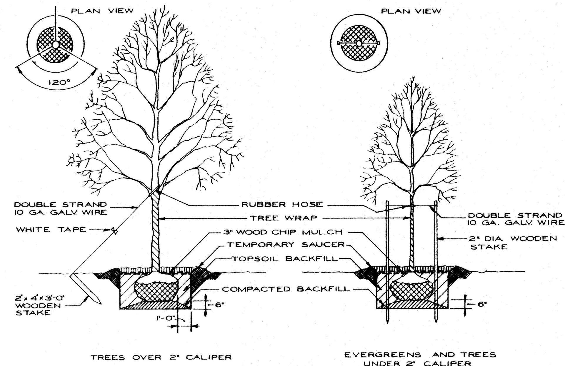
TREE GUYING AND STAKING DETAIL NO SCALE
