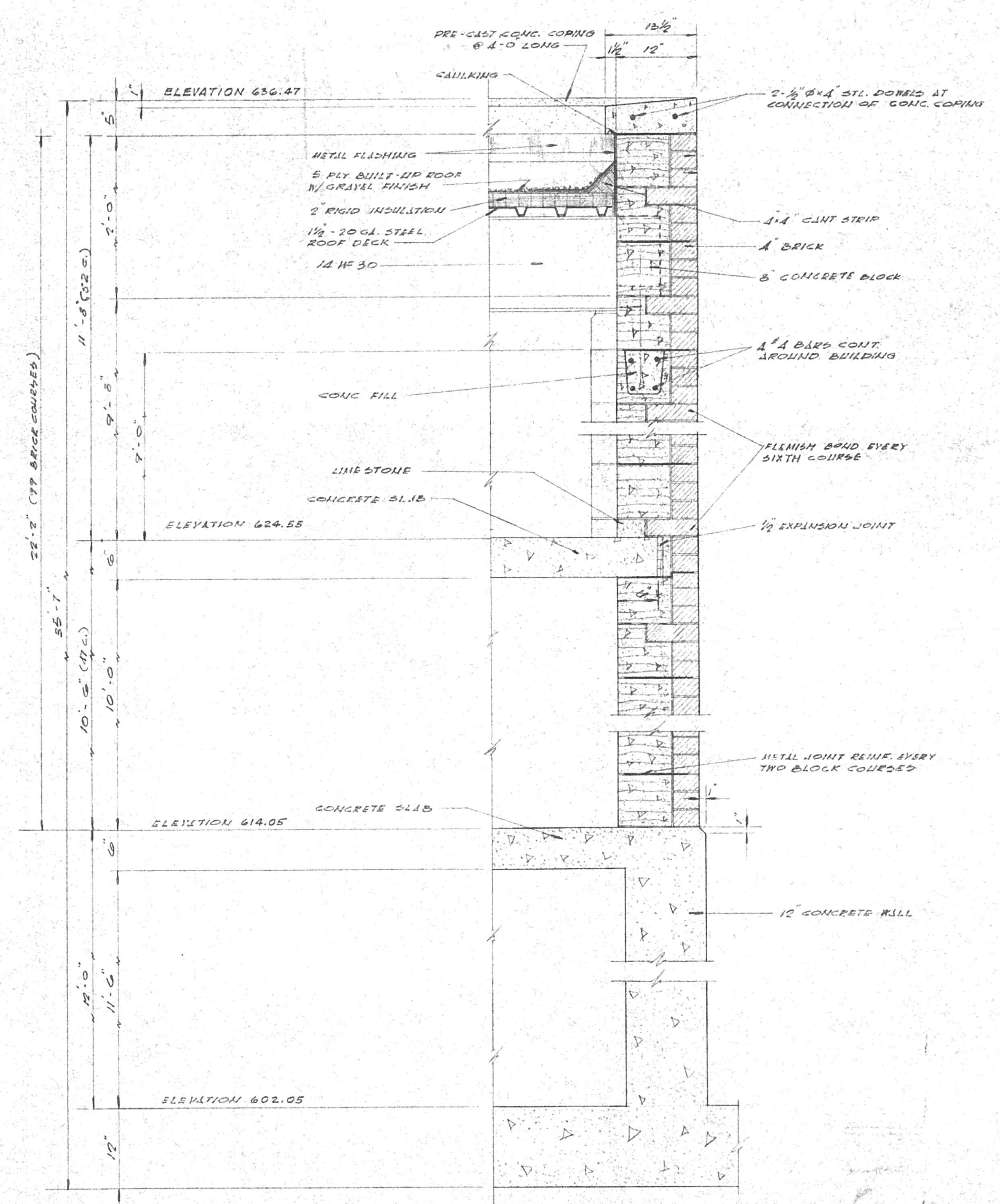
TYPICAL WALL SECTION SCALE: 1/2" = 1'-0"
