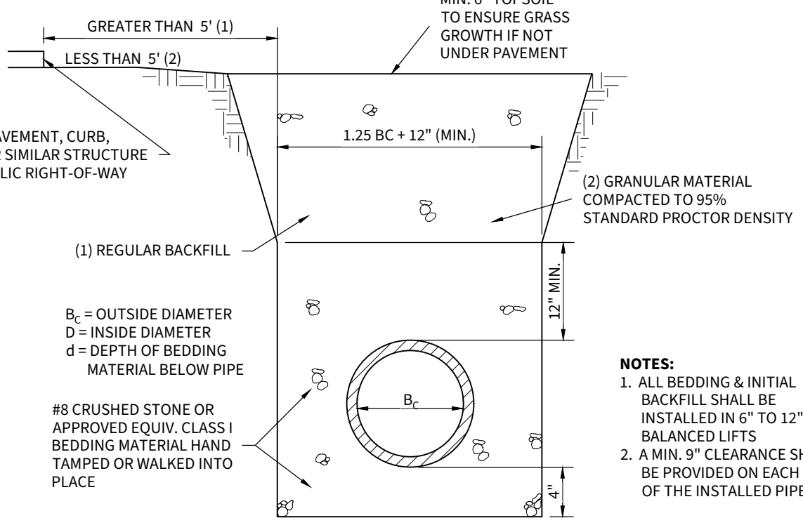
TYPICAL BEDDING SECTION - PVC & HDPE
