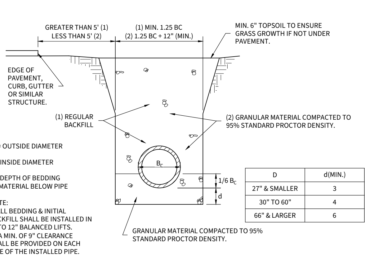
TYPICAL BEDDING SECTION - RCP PIPE
