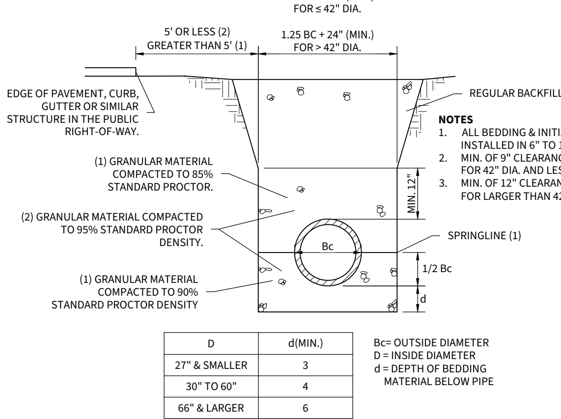
TYPICAL BEDDING SECTION - CMP
