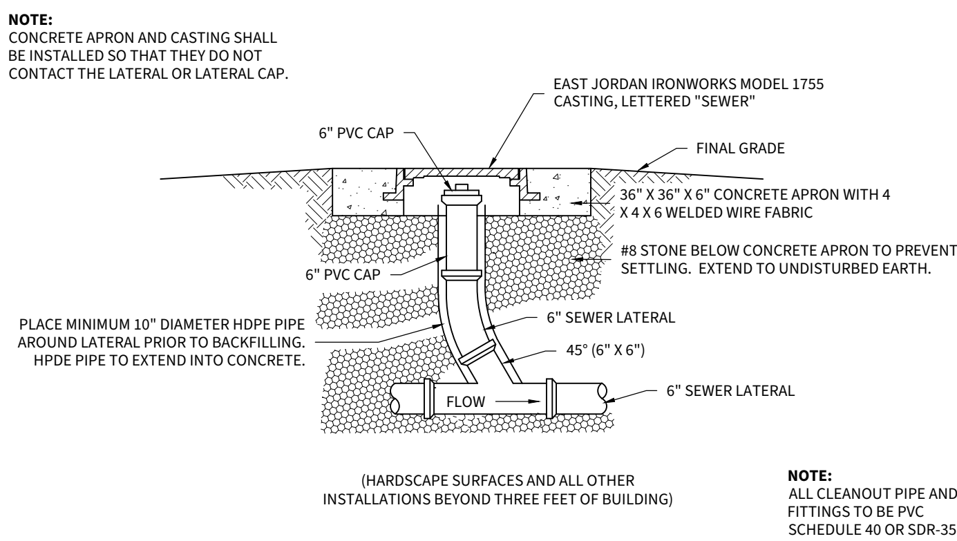
TYPICAL CLEANOUT SECTION
