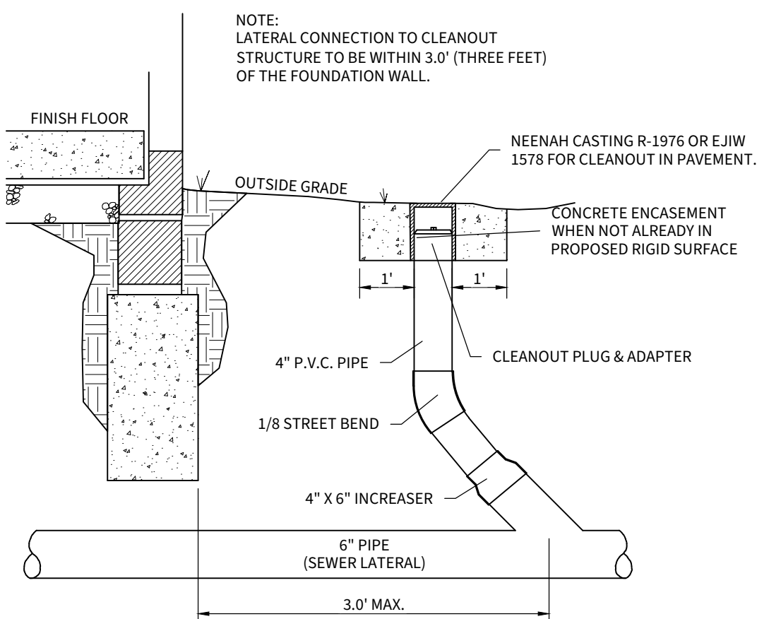
TYPICAL CLEANOUT SECTION
