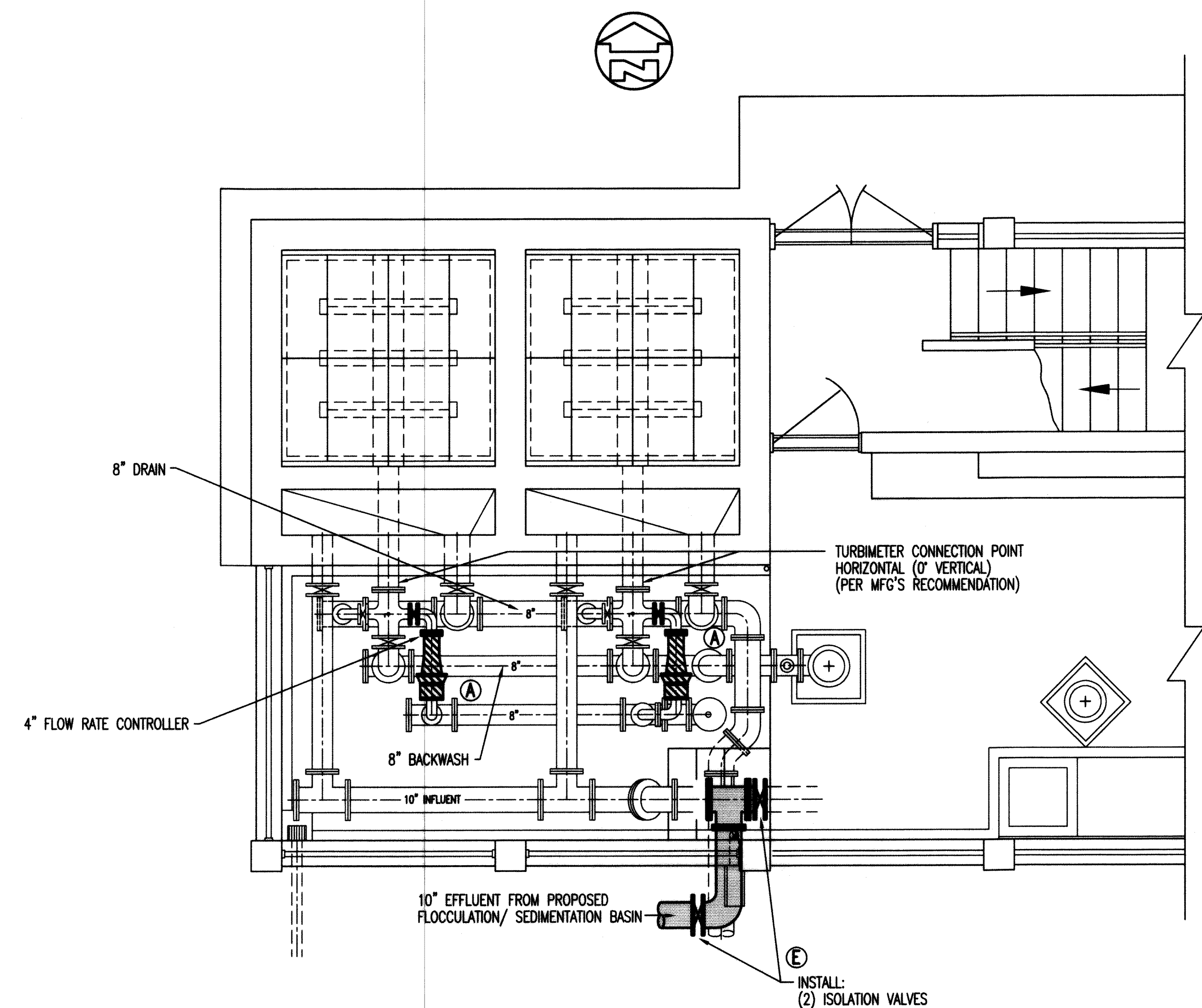
FIRST FLOOR PIPING PLAN SCALE: 3/8" = 1'-0"
