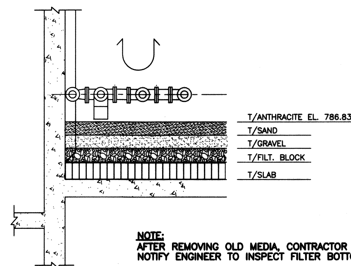
FILTER MEDIA DETAIL N.T.S.
