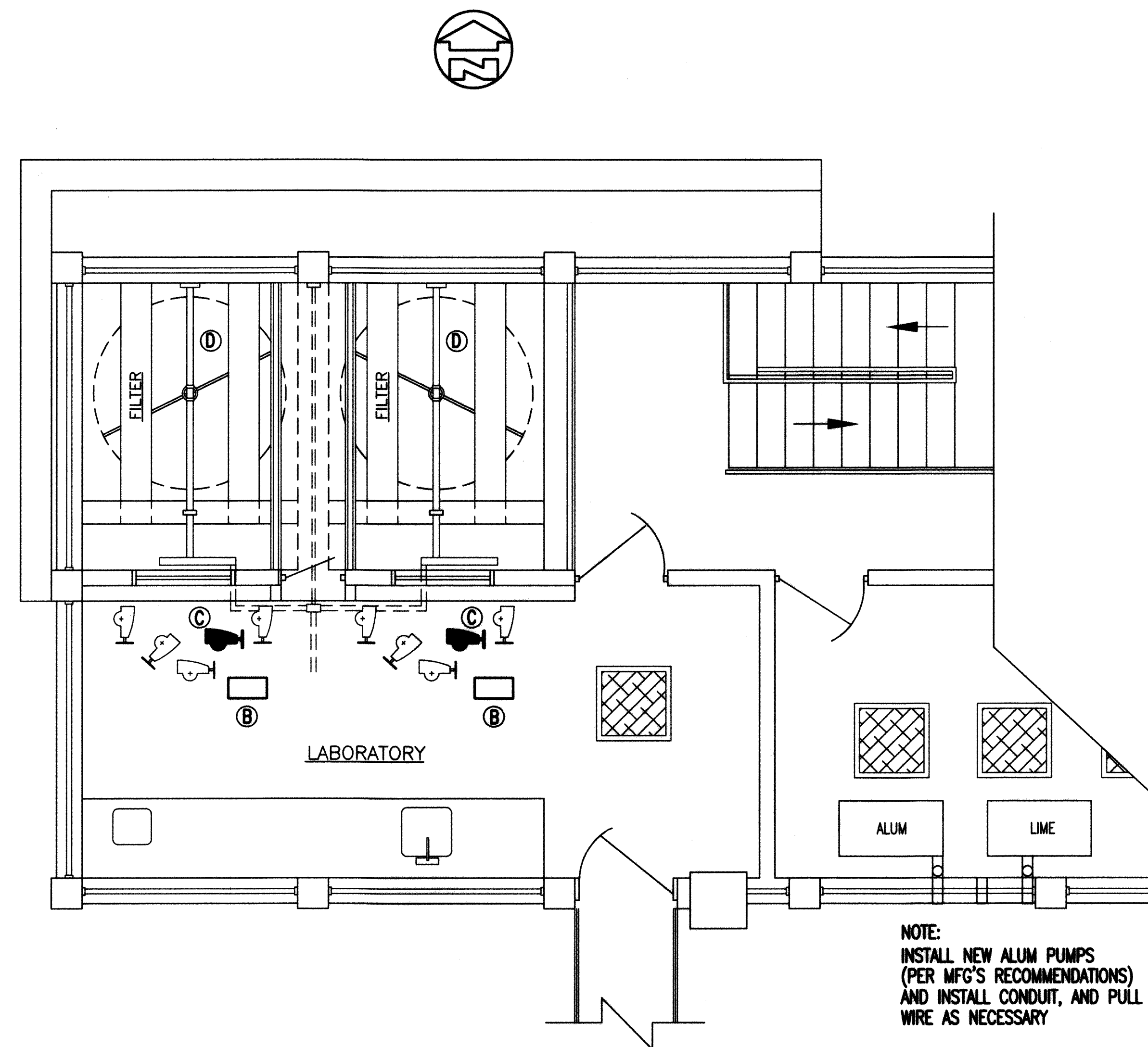
SECOND FLOOR PLAN LABORATORY AND FILTERS No. 1 & 2 SCALE: 3/8" = 1'-0"
