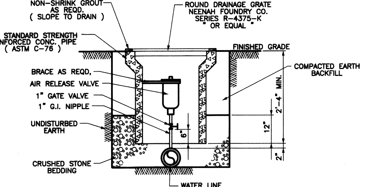
AIR RELEASE VALVE DETAIL NO SCALE
