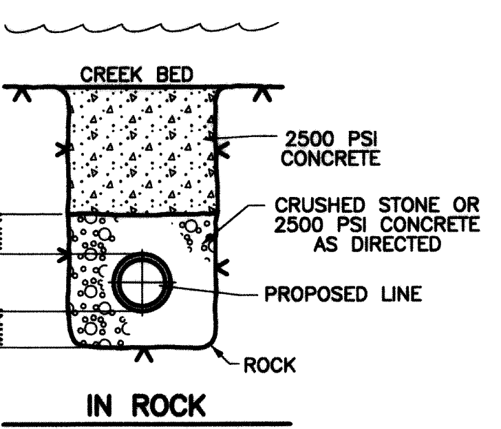
CREEK CROSSING DETAILS NO SCALE
