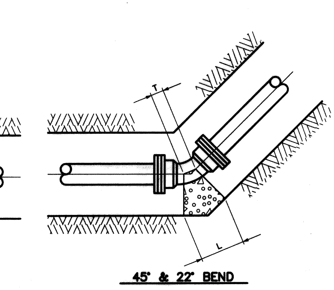
CONCRETE BLOCKING FOR FITTINGS NO SCALE
