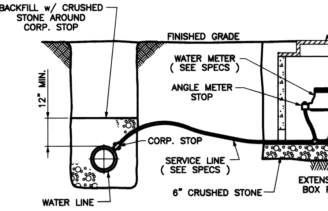
TYPICAL METER SETTING DETAIL NO SCALE
