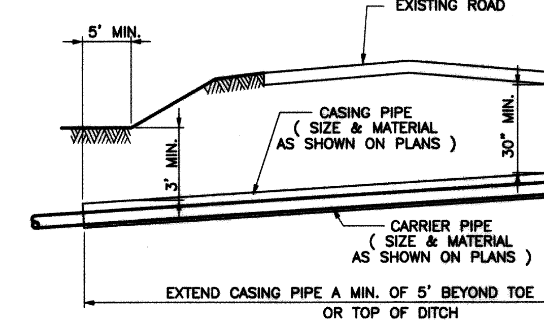
TYPICAL ROAD BORE DETAIL NO SCALE
