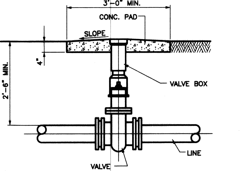
TYPICAL VALVE SETTING DETAIL NO SCALE
