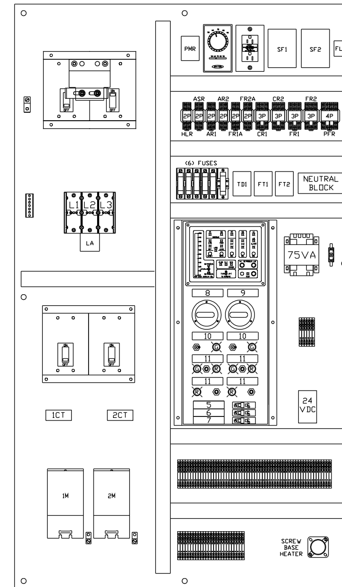
BACK PANEL LAYOUT 57"H x 33"W
