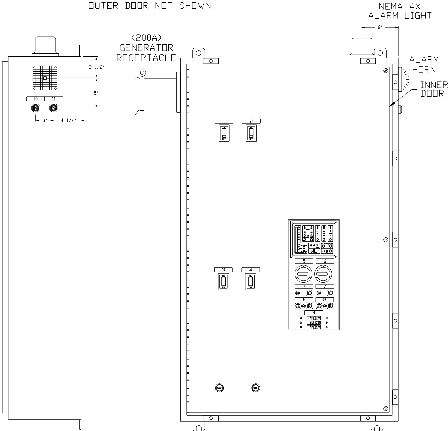
SIDE VIEW
