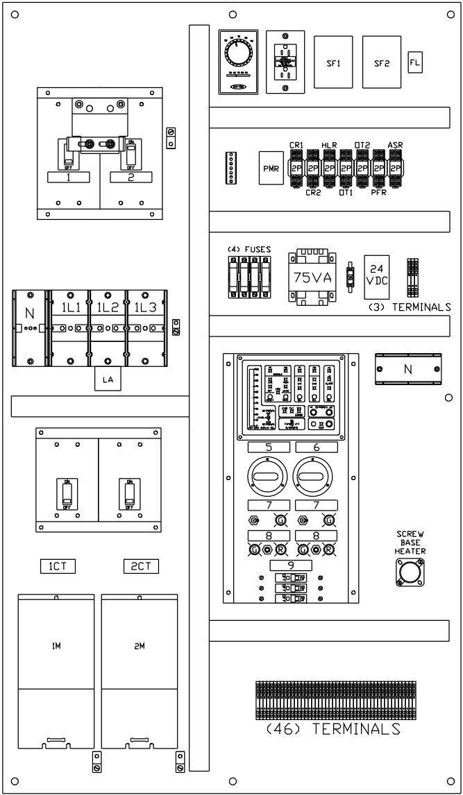
BACK PANEL LAYOUT 57"H x 33"W
