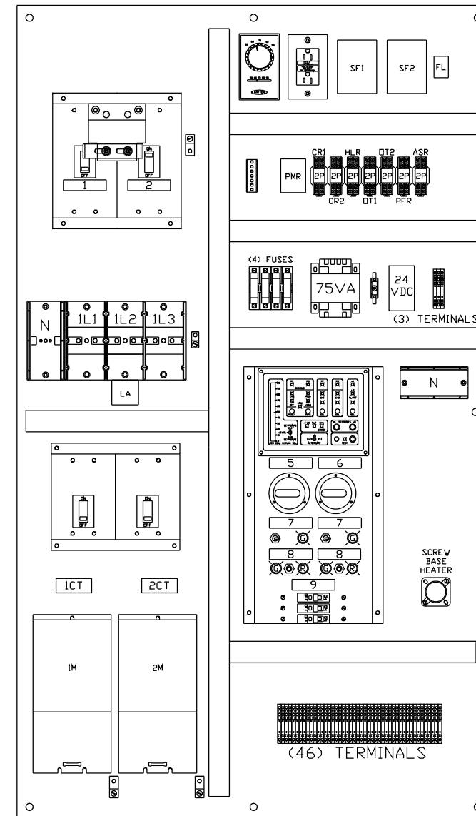
BACK PANEL LAYOUT 57"H x 33"W
