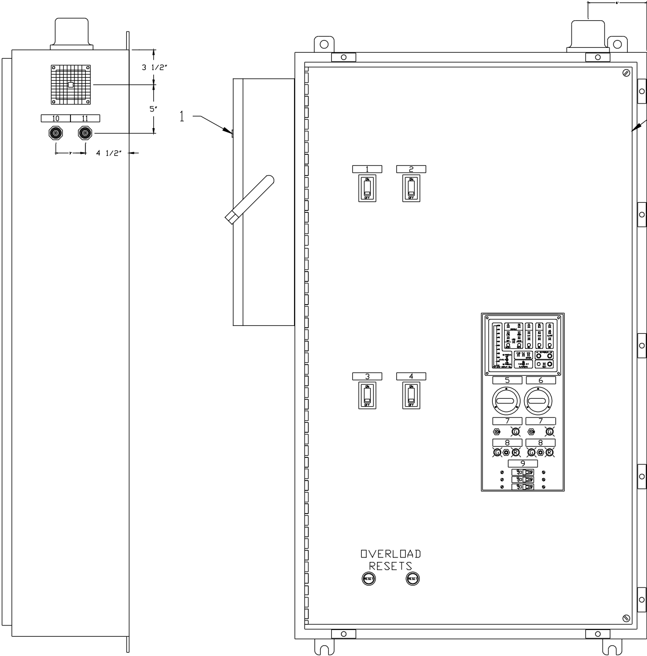
SIDE VIEW
