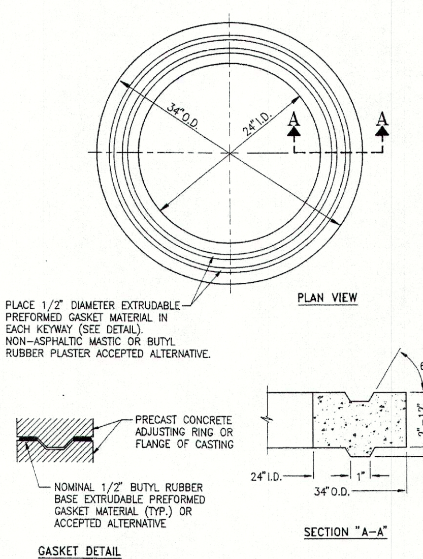
PRECAST CONCRETE ADJUSTING RING MADISON COUNTY HIGHWAY ENGINEER'S OFFICE
