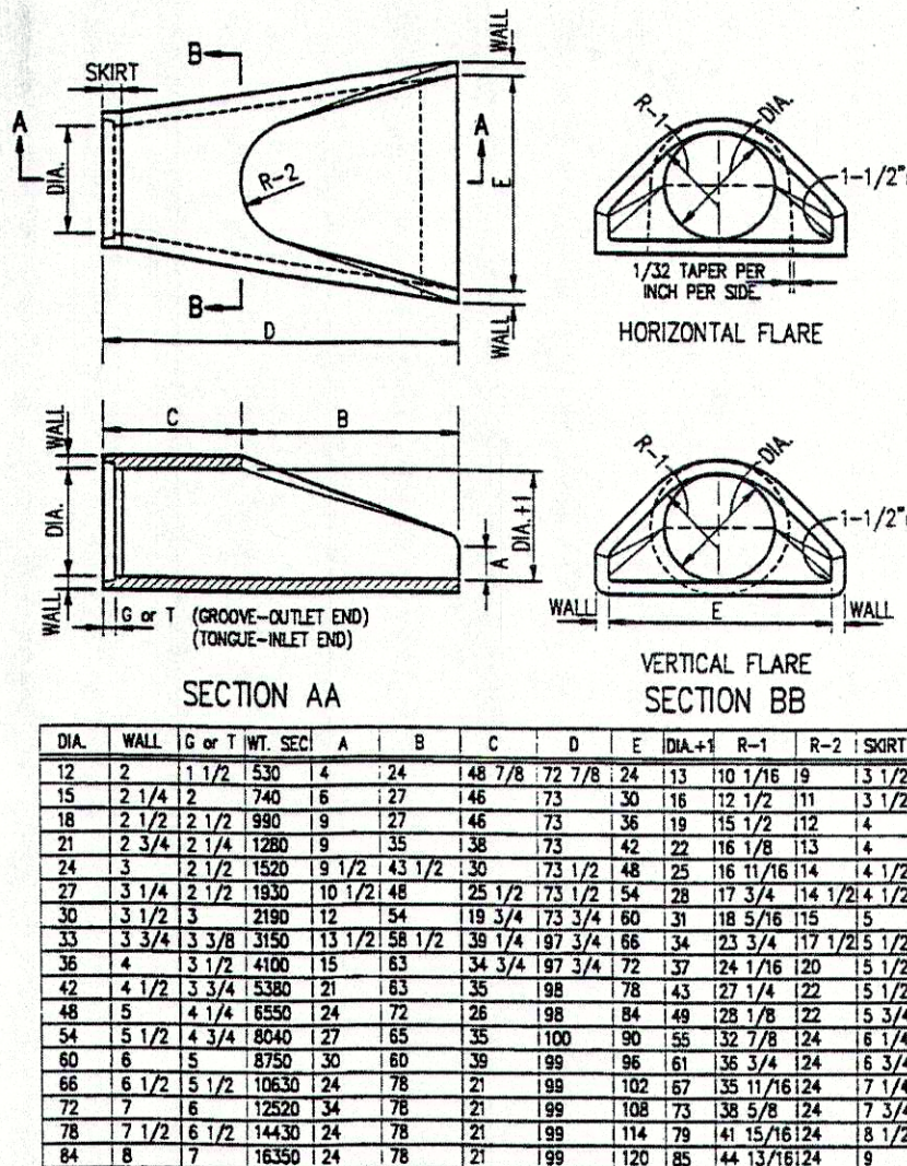
CONCRETE END SECTION MADISON COUNTY HIGHWAY ENGINEER'S OFFICE
