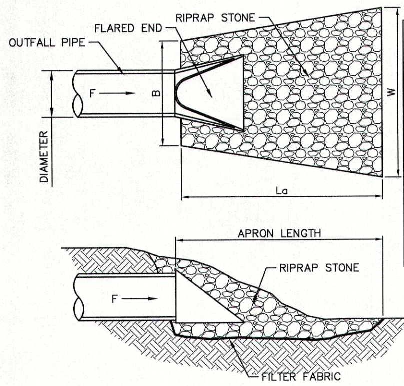
RIP-RAP PLACEMENT NOT TO SCALE
