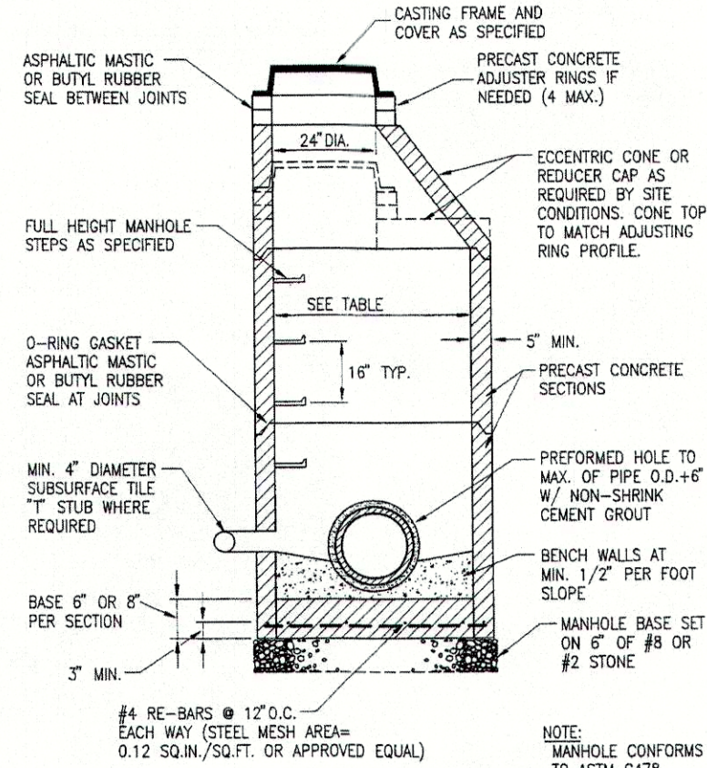
STANDARD DETAIL - MADISON COUNTY, INDIANA
