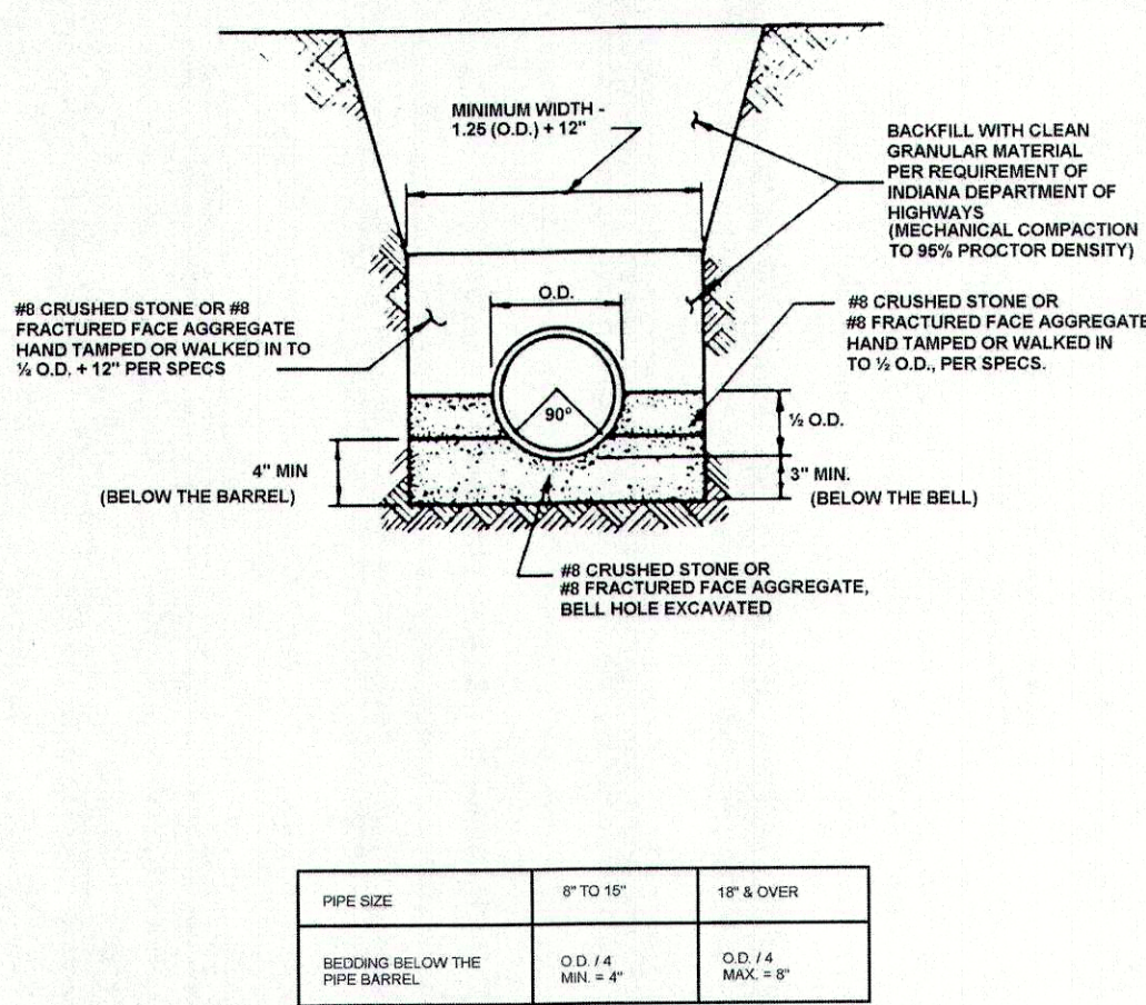
FLEXIBLE PIPE BEDDING DETAIL PVC & HDPE Pipe
