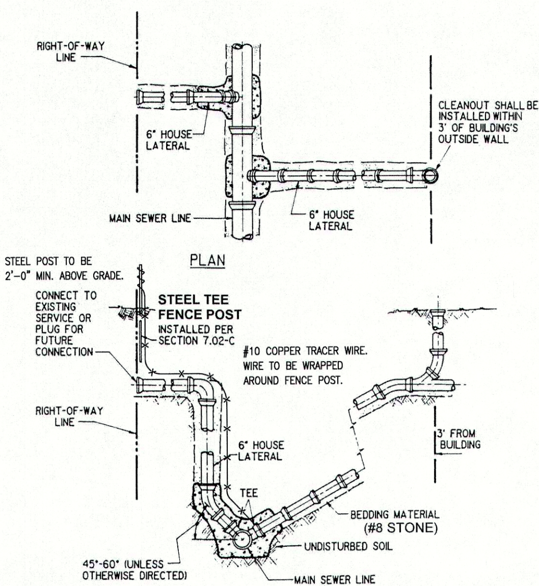
SERVICE CONNECTION FOR DEEP SEWERS ( 15' DEEP AND OVER )
