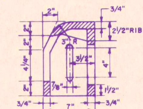
CURB CASTING SECTION CASTINGS TYPE 9 & 11
