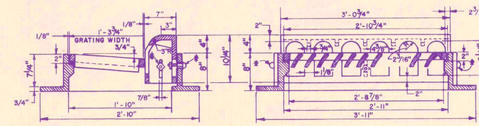
SECTION "A-A"
