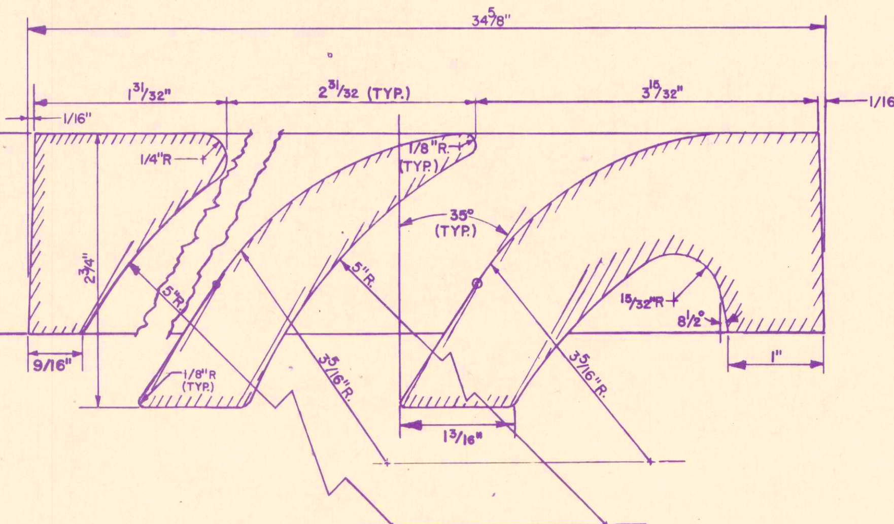
FIN DETAIL FOR CASTINGS TYPE 10 & 11
